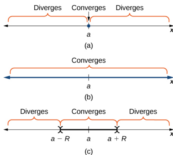
Figure 6.2 For a series \sum_{n=0}^{\infty} c_n(x - a)^n graph (a) shows a radius of convergence at R = 0 , graph (b) shows a radius of convergence at R = \infty , and graph (c) shows a radius of convergence at R . For graph (c) we note that the series may or may not converge at the endpoints x = a + R and x = a - R .
