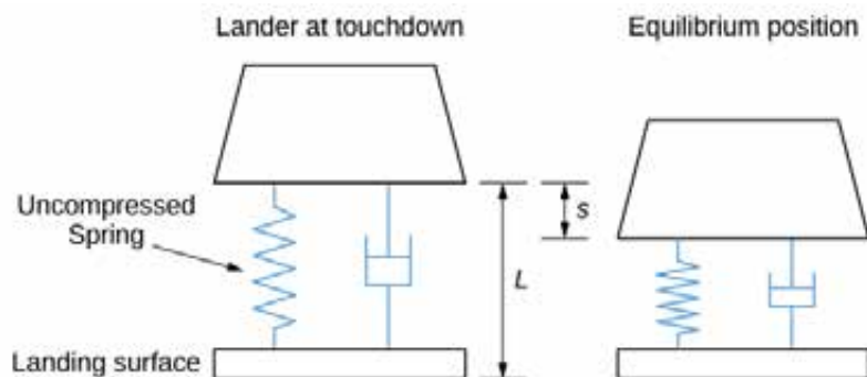
Figure 7.12 The landing craft suspension can be represented as a damped spring-mass system. (credit “lander”: NASA)
