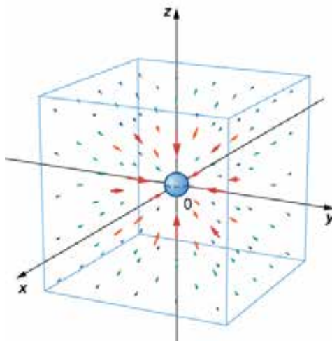
Figure 6.8 A visual representation of gravitational vector field \mathbf{F} = -Gm_1m_2 \left\langle \frac{x}{r^3}, \frac{y}{r^3}, \frac{z}{r^3} \right\rangle for a large mass at the origin.
