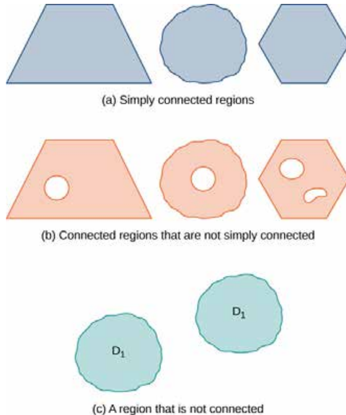
Figure 6.27 Not all connected regions are simply connected. (a) Simply connected regions have no holes. (b) Connected regions that are not simply connected may have holes but you can still find a path in the region between any two points. (c) A region that is not connected has some points that cannot be connected by a path in the region.
